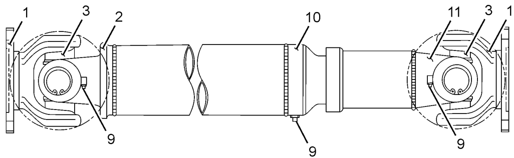
PROPELLER SHAFT REAR
